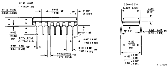
14-Lead Molded Dual-In-Line Package (N) Order Number DM74LS164N NS Package Number N14A
